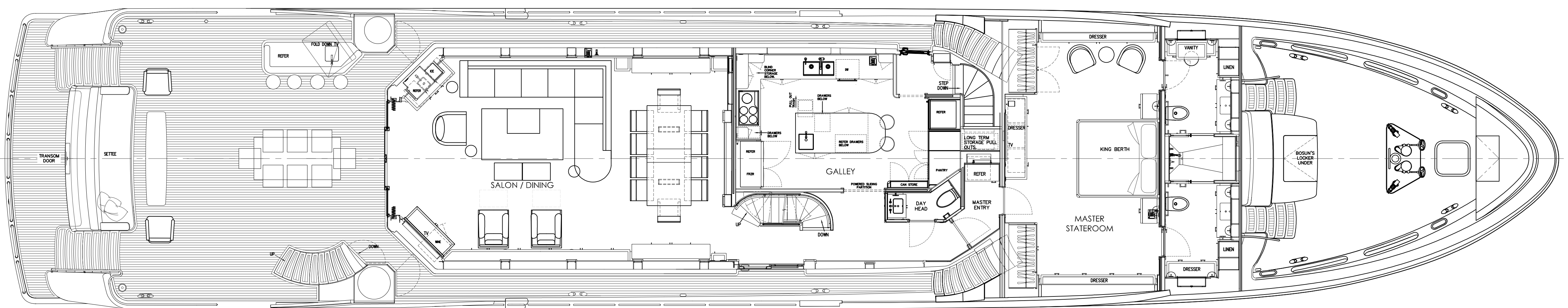
MAIN DECK
