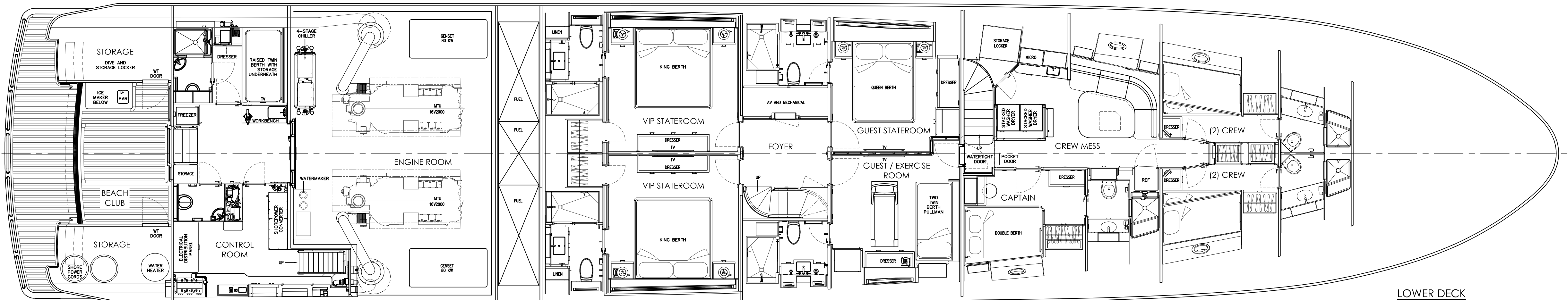
LOWER DECK
