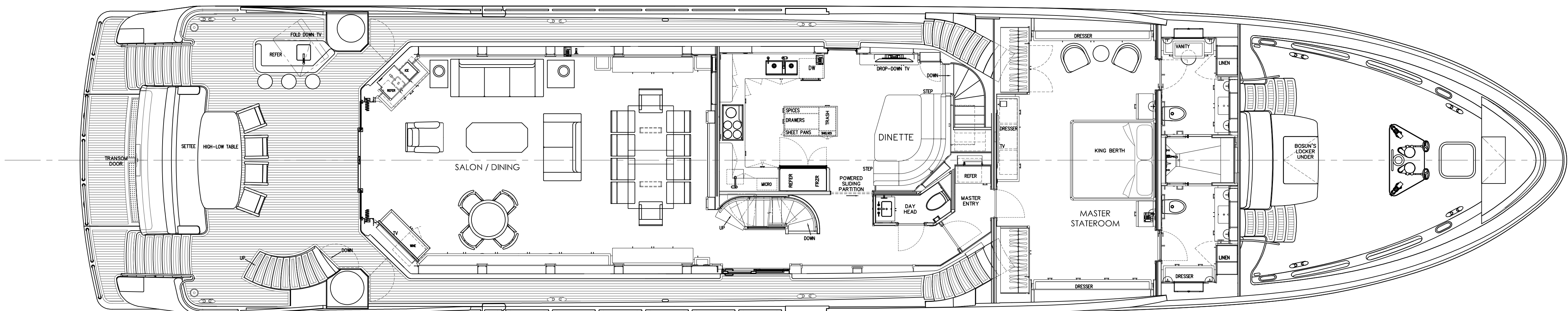
MAIN DECK
